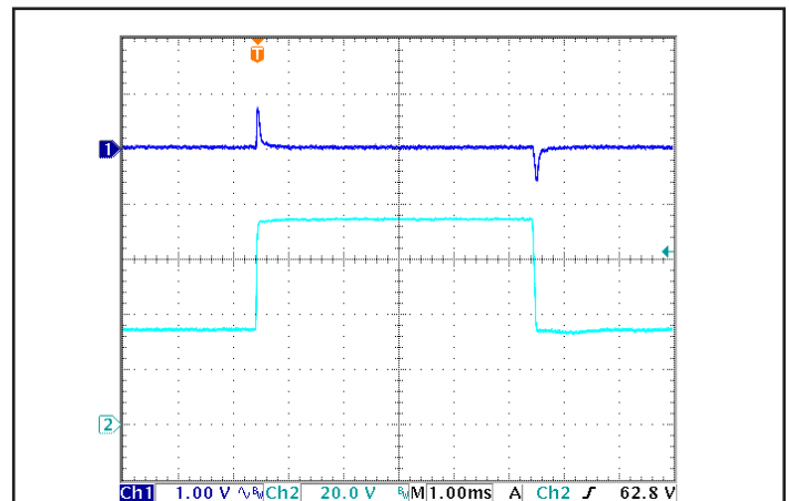
Figure 6: Output voltage response to step-change in input voltage (nominal to maximum, 1000 V/ms). Load cap: 15 \mu\text{F} tantalum and 1 \mu\text{F} ceramic capacitors. Ch 1: V_{out} , Ch 2: V_{in} .
