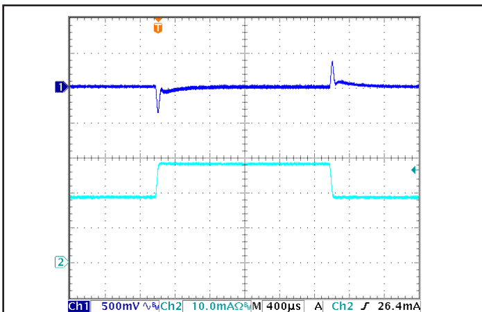
Figure 5: Output voltage response to step-change in load current (50% -75% -50% of I out (max); dI/dt = 0.1 A/μs). Load cap: 15 μF tantalum and 1 μF ceramic capacitors. Ch 1: V out , Ch 2: I out (5 A/div).
