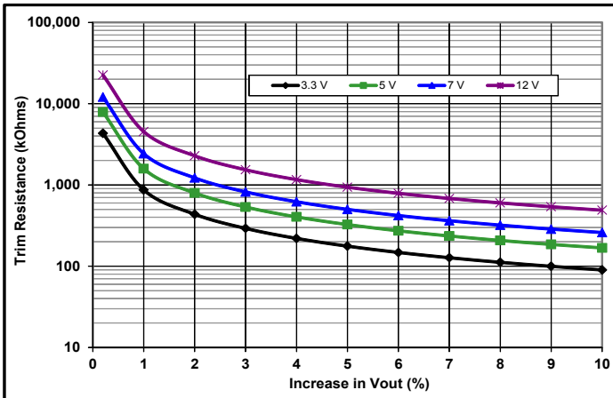
Common Figure 3: Trim graph for trim-up 3.3 to 12 V outputs.
